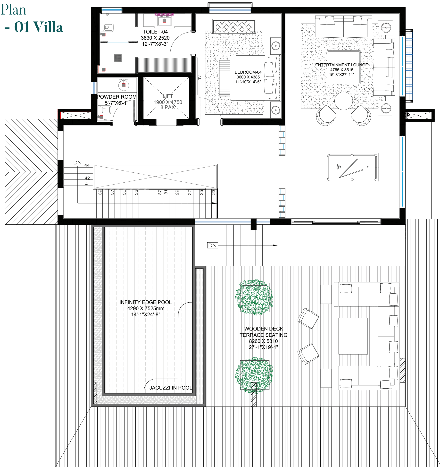
SECOND FLOOR VILLA TYPE-01
