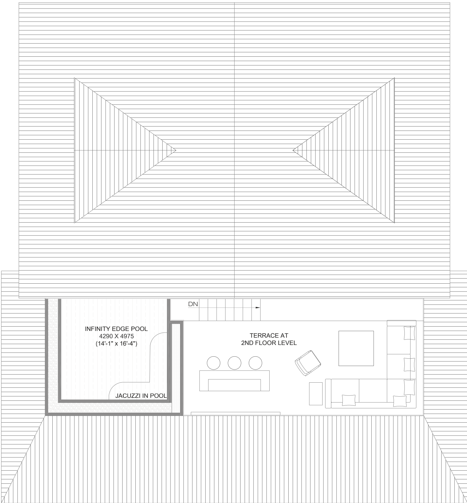
ROOF PLAN VILLA TYPE-02
