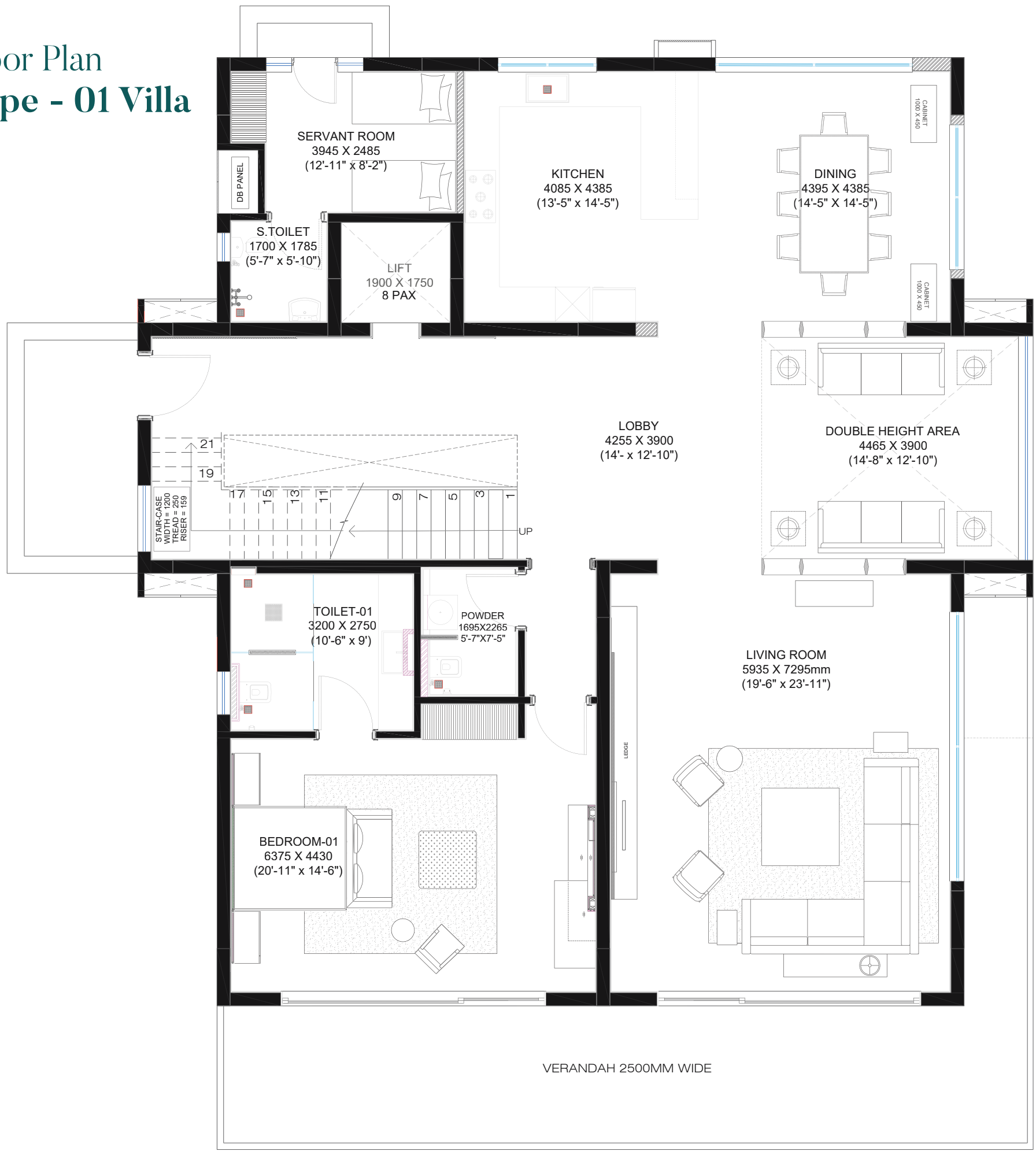
GROUND FLOOR VILLA TYPE-01
